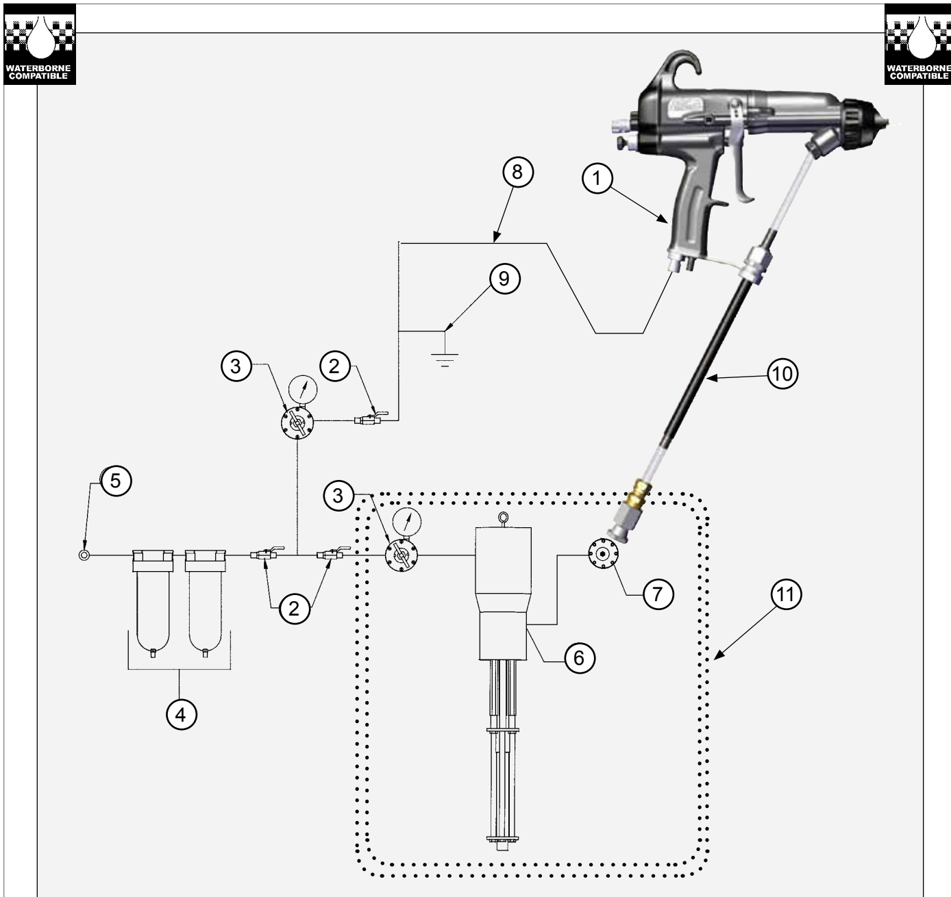
Figure 2: RansFlex Typical Waterborne Installation
